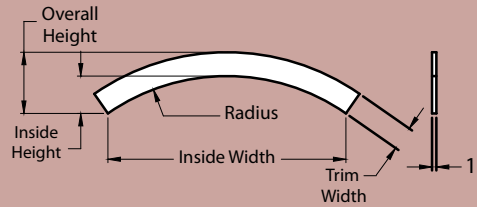
The 4F and 6F Segment Arches ship with angled ends, as shown by the dotted lines.
